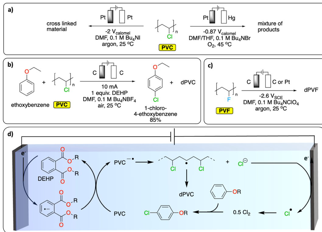
Fig. 9 Electrochemical dehalogenation. (a) Electrochemical degradation of PVC; (b) tandem electrochemical dechlorination of PVC with concomitant chlorination of an electron-rich arene; 85 (c) electrochemical defluorination of PVF; 89 (d) schematic representation of the DEHP-mediated reductive dichlorination of PVC coupled with chlorination of an electron-rich arene. The abbreviations dPVC and dPVF refer to (partial) dechlorinated PVC and (partial) defluorinated PVF, respectively. 85
