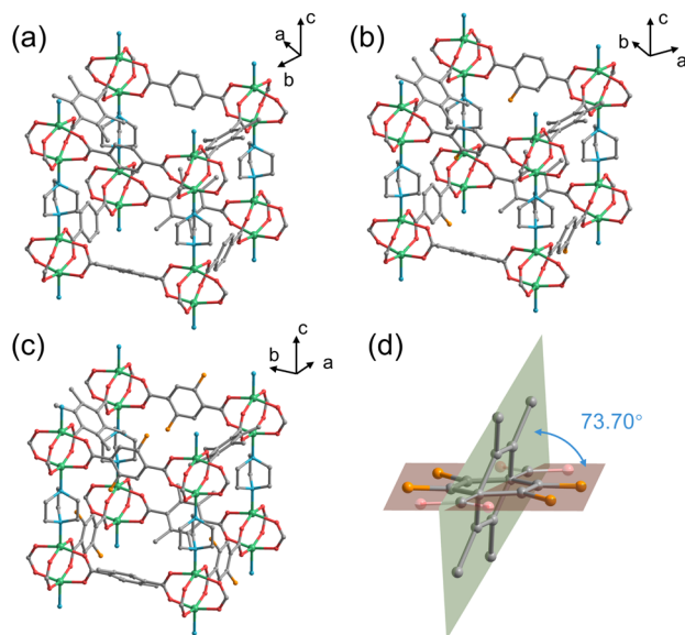
Fig. 1 Expanded cubic-like structure of (a) DMOF-0F , (b) DMOF-1F , and (c) DMOF-2F , in which only one orientation of the disordered xFBDC ligand is shown. (d) Disorder of 1FBDc and 2mBDc in DMOF-0F . Hydrogen atoms are omitted for clarity. Colour code: C: grey; F: orange; N: blue; O: red; Zn: green.
