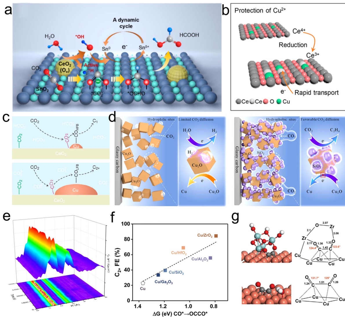
Fig. 9 (a) Proposed reaction mechanism of \text{CO}_2 to \text{HCOOH} on the \text{Sn}-\text{CeO}_2 surface. Reproduced with permission from ref. 118. Copyright 2023, American Chemical Society. (b) Scheme of the self-sacrifice mechanism to protect \text{Cu}^{2+} . Reproduced with permission from ref. 98. Copyright 2022, American Chemical Society. (c) Proposed \text{CO}_2\text{RR} mechanism at the \text{Cu} and \text{CeO}_2 interface. Reproduced with permission from ref. 119. Copyright 2022, American Chemical Society. (d) Schematic depiction of different catalytic microenvironments of \text{Cu}_2\text{O} and \text{Cu}_2\text{O}/\text{SiO}_2 . Reproduced with permission from ref. 123. Copyright 2023, American Chemical Society. (e) In situ EXAFS data of \text{CuSiO}_x during \text{CO}_2\text{RR} reaction at -1.4 V vs. RHE. Reproduced with permission from ref. 97. Copyright 2023, American Chemical Society. (f) The relationship between \Delta G of \text{*CO} to \text{*OCCO} and the Faraday efficiency of \text{C}_{2+} products for \text{Cu} and \text{Cu}/\text{oxide} catalysts. (g) The optimized configurations for \text{*OCCO} on \text{Cu} and \text{Cu}-\text{ZrO}_2 heterostructure. Reproduced with permission from ref. 22. Copyright 2022, Elsevier.
