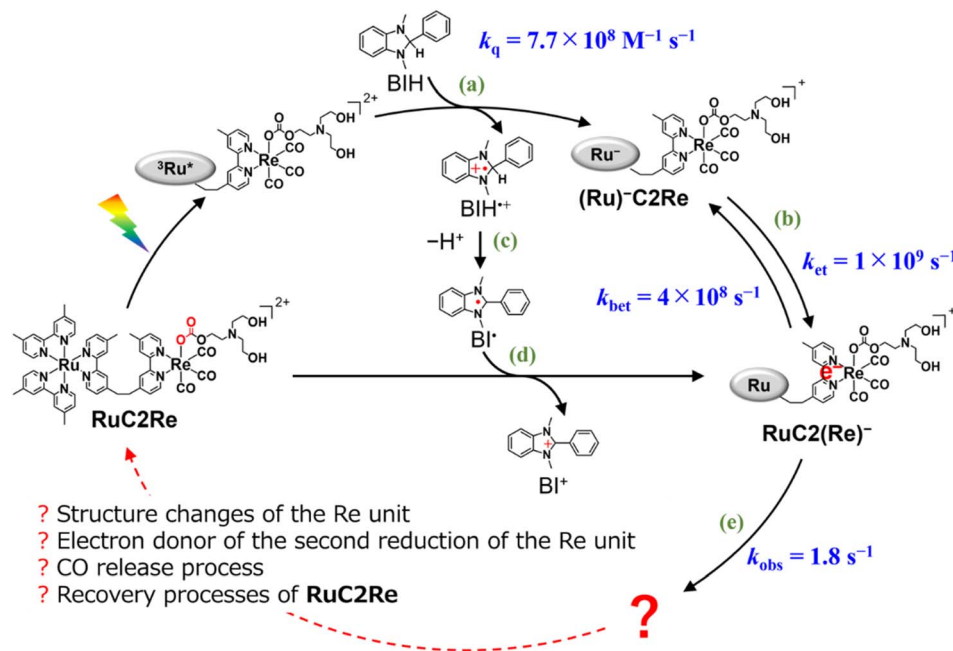
Scheme 1 Formation processes of the one-electron reduced species (OERS) of \text{RuC2Re} and unknown processes shown as “?”.
