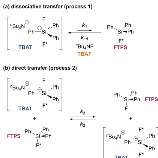
Scheme 2 Two limiting pathways of fluoride transfer from TBAT to FTPS. (a) Dissociative transfer via TBAF, where K_1 = k_1/k_{-1} \ll 1 . (b) Direct bimolecular transfer (the rate constants in each direction, k_2 , are identical, as \Delta G^\circ = 0 ). In each transfer pathway, examples of exchanging fluorine atoms are marked in bold with an asterisk.
