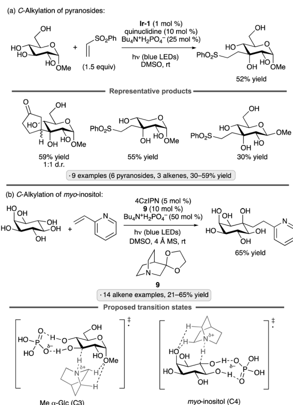
Scheme 51 Site-selective C -alkylations of pyranosides and myo-inositol, and proposed transition state structures for selective HAT. Ir-1 denotes [\text{Ir}(\text{d}(\text{CF}_3)_2\text{ppy})_2(\text{dtbbpy})]\text{PF}_6 ; 4CzIPN denotes 1,2,3,5-tetrakis(carbazol-9-yl)-4,6-dicyanobenzene.
