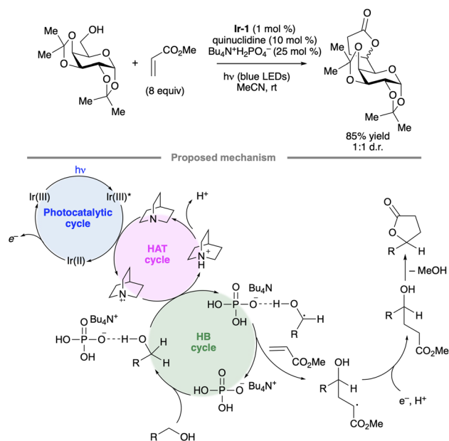
Scheme 50 Selective C -alkylation of a protected galactopyranose by photoredox/HAT/hydrogen bonding co-catalysis. Ir-1 denotes [\text{Ir}(\text{d}(\text{CF}_3)_2\text{ppy})_2(\text{dtbbpy})]\text{PF}_6 .
