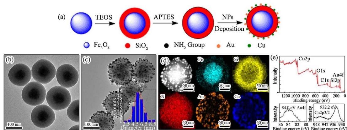
Fig. 6 (a) Stepwise preparation process of \text{Fe}_3\text{O}_4@(\text{SiO}_2-\text{Au/Cu}) magnetic nanocomposites. TEM images of (b) \text{Fe}_3\text{O}_4@(\text{SiO}_2) and (c) \text{Fe}_3\text{O}_4@(\text{SiO}_2-\text{Au/Cu}) nanoparticles. The inset in (c) depicts the nominal size distribution of Au/Cu NPs over the silica surface, determined by calculating the diameters of around 200 particles in the TEM images. (d) High-angle annular dark-field STEM image of the \text{Fe}_3\text{O}_4@(\text{SiO}_2-\text{Au/Cu}) nanocomposite, accompanied by the elemental mapping of Fe, Si, N, Au, and Cu and (e) XPS survey of the \text{Fe}_3\text{O}_4@(\text{SiO}_2-\text{Au/Cu}) nanocomposite and high-resolution Au 4f and Cu 2p spectra (adapted with permission from ref. 172, Elsevier, (2018)).
