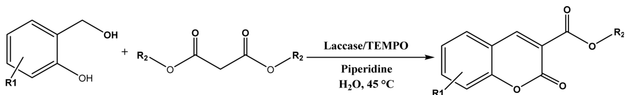
Fig. 29 One-pot synthesis of coumarin-3-carboxylates using laccase/TEMPO hybrid catalyst.
