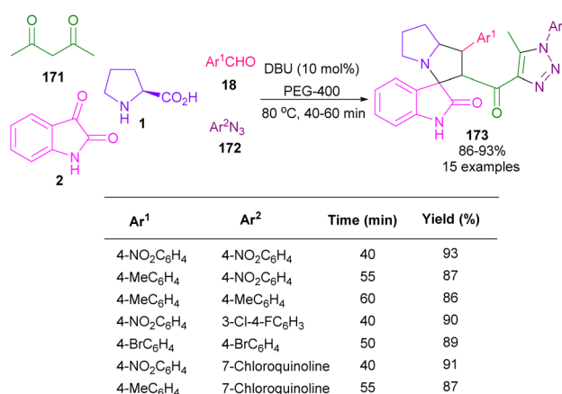
Scheme 48 Multi-component reaction of isatin, L-proline, aryl azides, aryl aldehydes, and acetylacetone.
