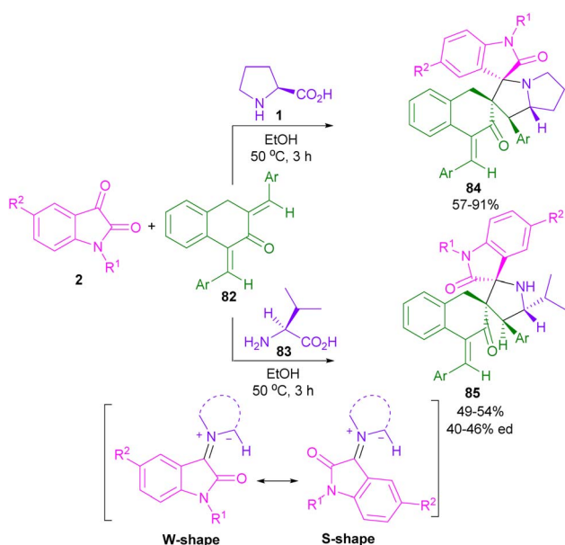
Scheme 25 Reaction of isatins, amino acids and p -substituted 1,3-bis(arylidene)tetra-2-ones.
