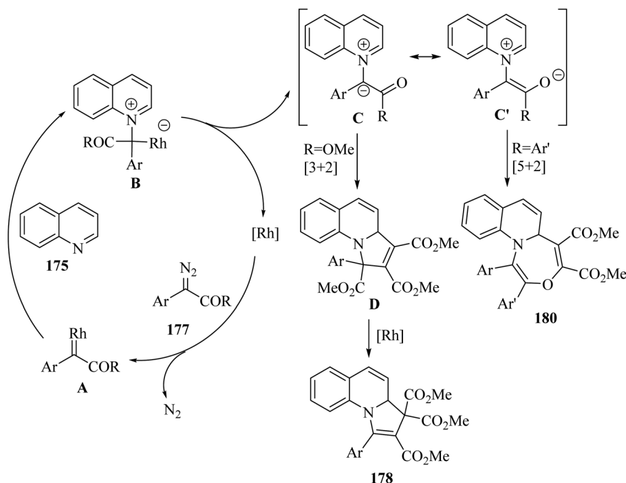
Scheme 77 Possible reaction mechanism for the synthesis of seven-membered 1,4-oxazepines 180 and five-membered indolizines 178 . 85
