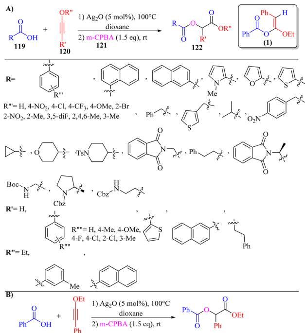
Scheme 55 (A) Ag 2 O catalyzed synthesis of \alpha -carboxyloxy esters 122 . (B) Gram-scale reaction for the synthesis of \alpha -carboxyloxy ester; 1 : \alpha -alkoxy enol ester intermediate synthesized via the reaction between benzoic acid and enol ether. 71
