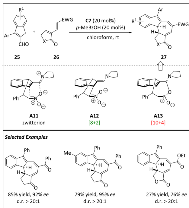
Scheme 9 Asymmetric intermolecular [10 + 4] cycloadditions via the isobenzofulvene intermediate.
