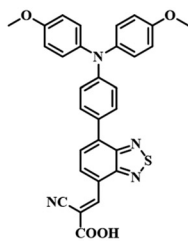
(28) MPA-BT-CA (PCE=21.24%)
