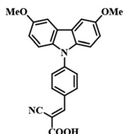
(31) Cz-CA (PCE=20.17%)
