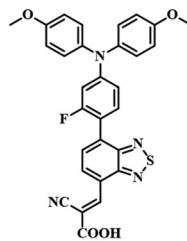
(29) FMPA-BT-CA (PCE=22.37%)
