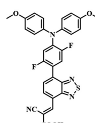
(30) 2FMPA-BT-CA (PCE=21.68%)
