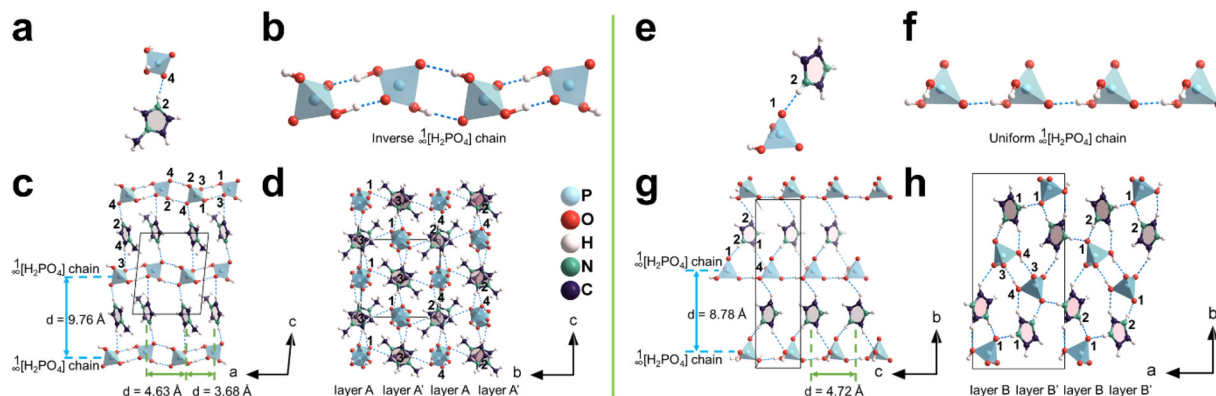
Fig. 2 Diagrams of (\text{C}_4\text{H}_7\text{N}_2)(\text{H}_2\text{PO}_4) structure: (a) asymmetric unit. (b) Inverse {}^\infty[\text{H}_2\text{PO}_4] chain. (c) Pseudo 2D intercalated structure in the ac plane. (d) 3D structure viewed in the bc plane. Diagrams of (\text{C}_3\text{H}_5\text{N}_2)(\text{H}_2\text{PO}_4) structure: (e) asymmetric unit. (f) Uniform {}^\infty[\text{H}_2\text{PO}_4] chain. (g) Pseudo 2D intercalated structure in the bc plane. (h) 3D structure viewed in the ab plane.
