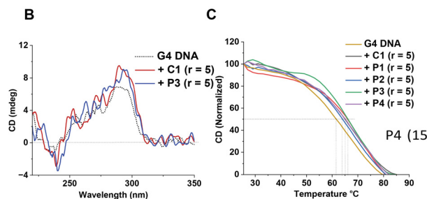
Fig. 2 (A) Chemical structure of NA-TACs ( P1–P4 ) and their control compound C1 . (B) CD spectra of 3 \mu M Hum 21-mer G4 DNA alone, with compound C1 and with P3 (15 \mu M) in 10 mM Tris-HCl (pH 7.4) containing 0.1 M KCl and 0.1 mM EDTA. (C) CD melting profiles of the pre-formed Hum 21-mer G4 DNA alone, and G-quadruplex DNA incubated with ligands C1 , P1 , P2 , P3 , and P4 (15 \mu M) in 10 mM Tris-HCl (pH 7.4) containing 0.1 M KCl and 0.1 mM EDTA.
