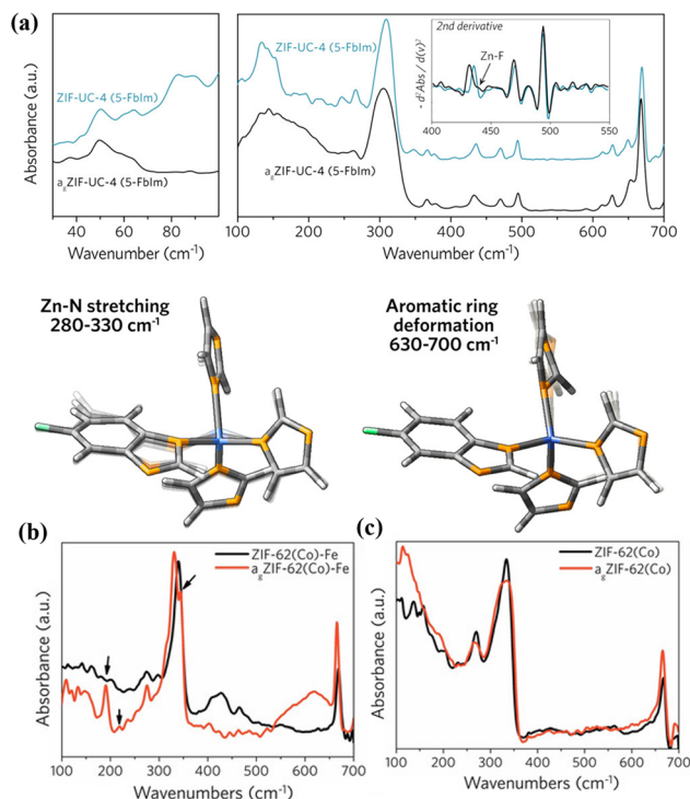
Fig. 7 (a) Structure comparison of MOF crystals and glass by THz/far-IR and the modes of ZnIn 3 S 2 -Fblm tetrahedra and aromatic rings utilized in DFT calculations. Reproduced with authorisation from ref. 65 and copyright 2020 by American Chemical Society. THz/Far-IR spectra of the vitrification for (b) ZIF-62(Co)-Fe and (c) ZIF-62(Co). Reproduced with authorisation from ref. 66 and copyright 2022 by Wiley-VCH GmbH.
