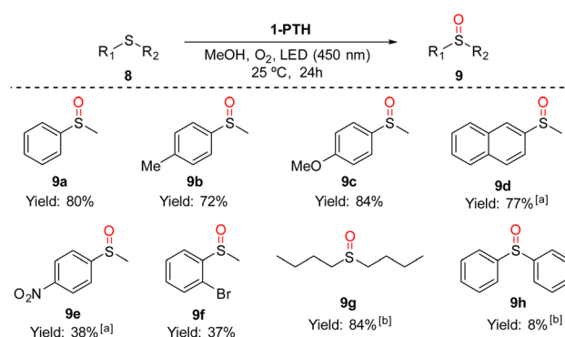
Scheme 5 Reaction conditions: sulphide 8 (0.1 mmol), film 1-PTH (0.6 mg) in methanol (200 \mu L) under an oxygen atmosphere was irradiated under 450 nm light for 24 h at rt. Isolated yields are obtained after purification by column chromatography. (a) 400 \mu L of methanol were used. (b) Yield determined by ^1\text{H} NMR using 1,3,5-trimethoxybenzene as the internal standard.
