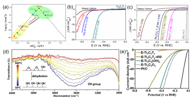
Fig. 3 (a) Volcano curve of exchange current as a function of the average Gibbs free energy of hydrogen adsorption. 44 Copyright 2017, American Chemical Society. LSVs of (b) \text{Ti}_3\text{C}_2\text{T}_x and (c) \text{Mo}_2\text{CT}_x in 0.5 M \text{H}_2\text{SO}_4 electrolyte. 45 Copyright 2018, American Chemical Society. (d) Magnified in situ temperature-dependent FTIR spectra of the as-synthesized \text{E-Ti}_3\text{C}_2(\text{OH})_x in Ar atmosphere; (e) polarization curves of various MXene. 47 Copyright 2019, Wiley.
