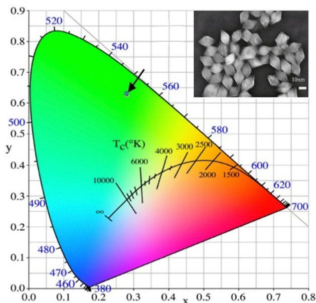
Fig. 12 The CIE chromaticity diagram of \text{Li}(\text{Gd,Y})\text{F}_4:\text{Yb,Er} (inset: the TEM image of \text{Y}^{3+} -doped \text{LiGdF}_4:\text{Yb}^{3+},\text{Er}^{3+} upconversion nanocrystals). Reprinted with permission from Elsevier. 68
