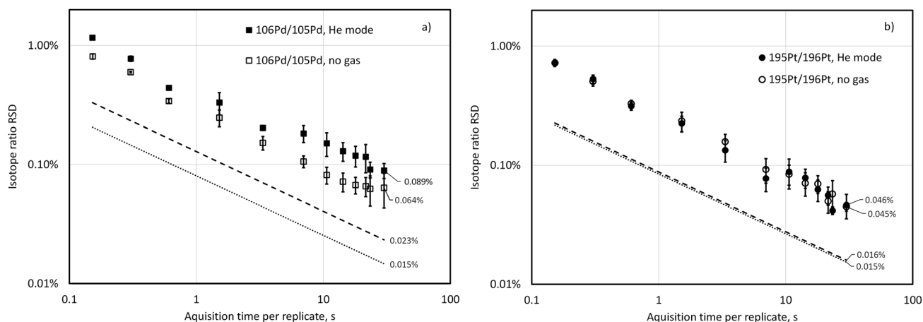
Fig. 1 Isotope-ratio RSD for ^{106}\text{Pd}/^{105}\text{Pd} (a) and ^{195}\text{Pt}/^{196}\text{Pt} (b) isotopic pairs when analysing a blend containing about 50 ng g -1 Pd and Pt, either using 2 mL min -1 He (closed symbols) or no gas (open symbols) in the CRC and standard sample introduction system. RSD are calculated for 10 consecutive replicates in continuous acquisition. Error bars are 1sd for 3 independent experiments conducted on the same day, about 40 min apart. Poisson limits of RSD are shown by a dotted (no-gas mode) or dashed line (He mode).
