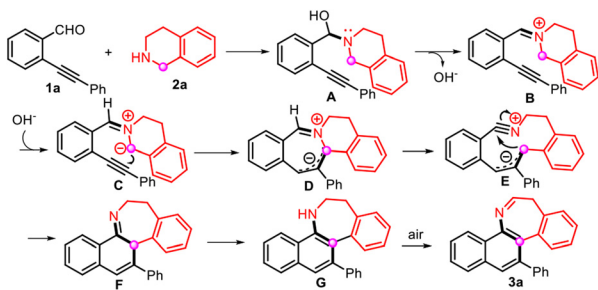
Scheme 2 Proposed mechanism.
