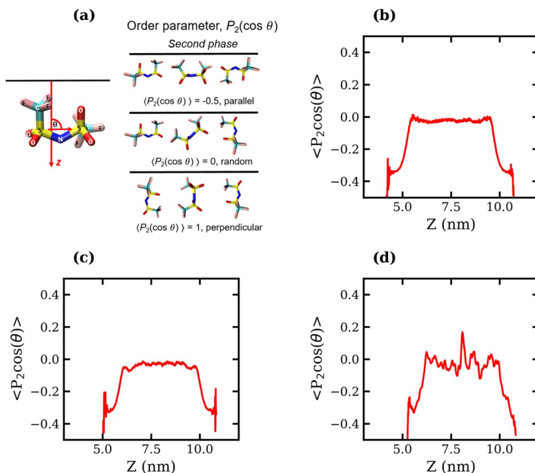
Fig. 5 Average order parameter, \langle P_2(\cos \theta) \rangle , of \text{TFSI}^- anions measured as the second Legendre polynomial of \theta , the angle between the S–S vector and interface normal (a), plotted against the Z coordinate for the (b) 1 molal, (c) 10 molal and (d) 20 molal liquid–vapour systems.
