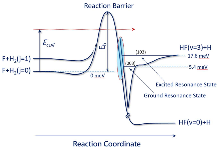
Fig. 3 Reaction resonances in the F + H_2 reaction. This figure presents the accurate physical picture of the quantum resonances in the F + H_2 ( j = 0 ) and F + H_2 ( j = 1 ) reactions, resembling a vibrationally excited HF molecule in the presence of an H atom. Two resonance states reside in the exit channel: the ground resonance state (003) at 5.4 meV is mainly responsible for the F + H_2 ( j = 0 ) reaction at temperatures below 40 K, while the excited resonance state (103) at 17.6 meV plays a more important role for the F + H_2 ( j = 0 ) reaction at temperatures above 40 K (adapted from ref. 200).
