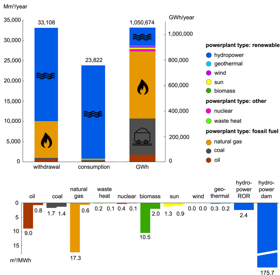
Fig. 1 (Top) Water withdrawal (WW) and consumption (WC) per powerplant fuel for the whole of Africa (in million m³ per year or Mm³ per year) as well as the related electricity produced in GWh. (Bottom) Average water intensity (WW and WC) per powerplant fuel for Africa (in m³ MWh⁻¹). Note that these are average values for all 2534 power plants, whereas individual plants show a wide range (range of values shown in Table 3).
