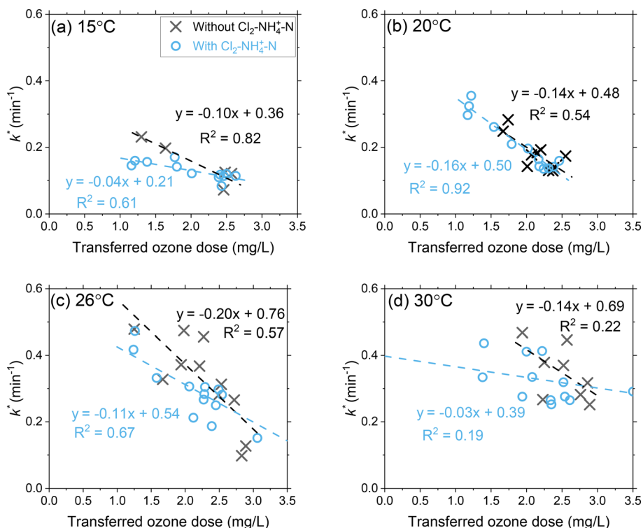
Fig. 3 Pilot-scale data depicting the correlations between the first-order ozone decay rate constants as a function of the transferred ozone dose at (a) 15 ^\circ\text{C} , (b) 20 ^\circ\text{C} , (c) 26 ^\circ\text{C} , and (d) 30 ^\circ\text{C} . Pilot-scale results illustrating the different \text{Cl}_2\text{-NH}_4^+\text{-N} dosing scenarios are presented in Fig. S6†. Another representation of the data in terms of the effect of transferred ozone doses on ozone half-life for all tested temperatures is shown in Fig. S7†.
