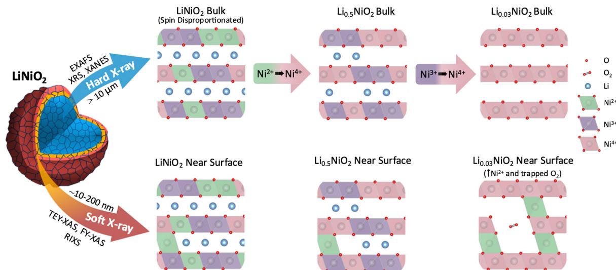
Fig. 6 Schematic representation of LiNiO 2 bulk charge compensation mechanism and surface degradation processes probed by different X-ray spectroscopy techniques. The differences in LiNiO 2 delithiation occurring at the surface and in the bulk, including the accommodation of trapped O 2 in pores formed near the surface by Ni 2+ species migrating to the Li layer. Continuous oxidation of Ni in bulk LiNiO 2 at high SoC is distinguished from the near surface degradation.
