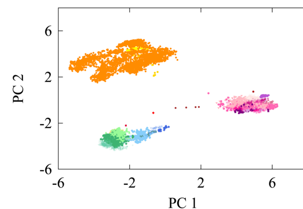
Fig. 3 (a) PCA of Oxygen-type embedding vectors of QM9-trained SchNet labelled according to Fig. 2b. The focus is on straight-chain alcohols. It can be seen even in the 2D projection that distances between the alcohols' embeddings converge as the chain gets larger. The Euclidean distance does indeed decrease for each successively larger straight-chain alcohol in the full PCA space. In that space, the distances between methanol, ethanol, propanol, butanol, and pentanol are 3.98, 2.12, 1.45, and 0.98, respectively. (b) PCA of oxygen-type embedding vectors of pretrained AIMNet neural net tested on the same QM9 dataset labelled according to Fig. 2b.
