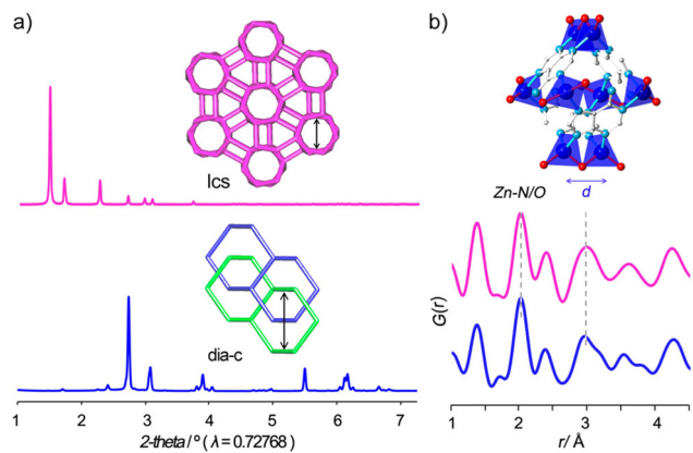
Fig. 9 (a) PXRD data of the bio-MOF-100 frameworks showing the occurrence of different crystalline phases and (b) PDF data showing the presence of the characteristic local structure in both phases. Reproduced with permission from ref. 63. Copyright 2017 American Chemical Society.
