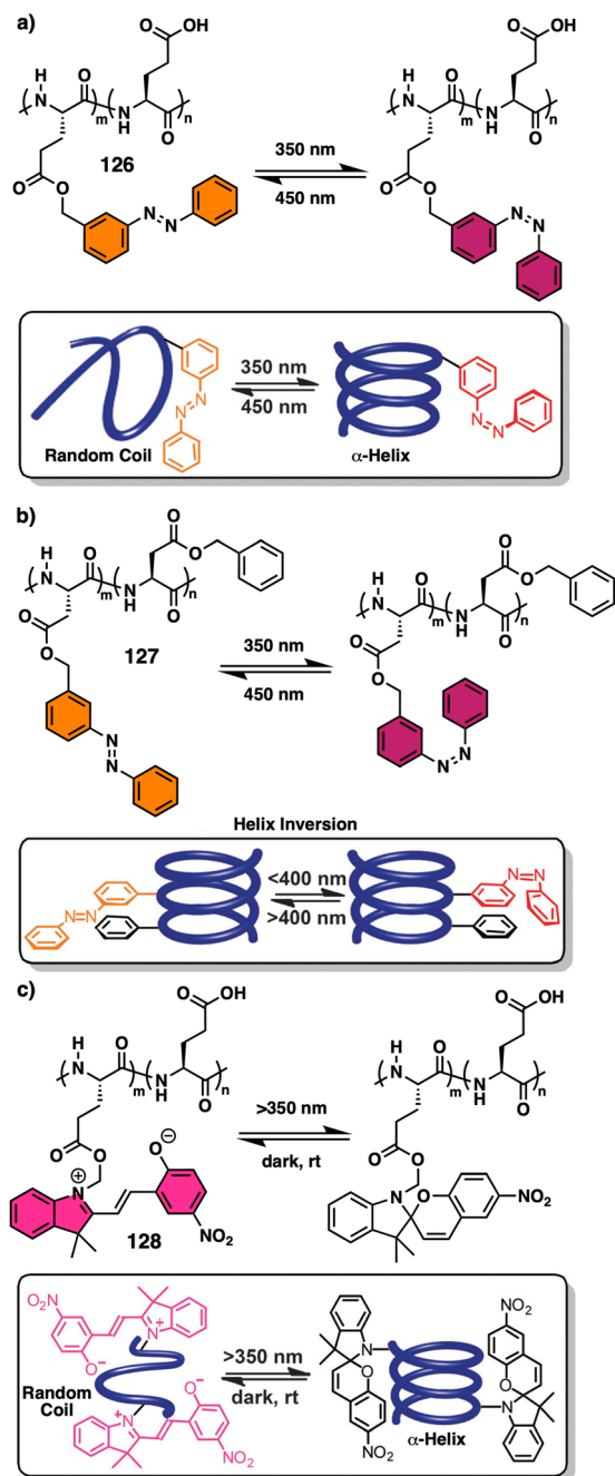
Fig. 60 Structure and behavior with light of \alpha -helical foldamers composed by (a) glutamic acid-azobenzene derivatives ( 126 ) and (b) aspartic acid-azobenzene derivatives ( 127 ). (c) Structure of glutamic acid-spiropyran derivative ( 128 ). A schematic illustration of the photoisomerization impact on the folding of the molecules is depicted below each section. Reproduced from ref. 295 with permission from the Royal Society of Chemistry, copyright 2016.
