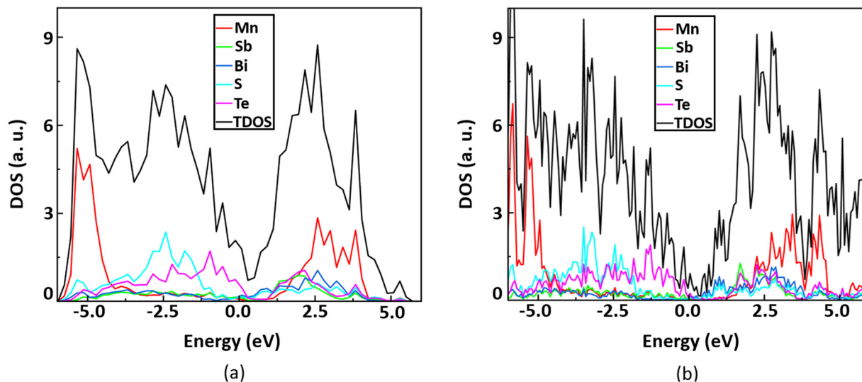
Fig. 3 The total density of states and the projected density of states of the monolayer MnSbBiS 2 Te 2 using (a) DFT+ U , and (b) HSE method. The Fermi level is set to 0 eV.
