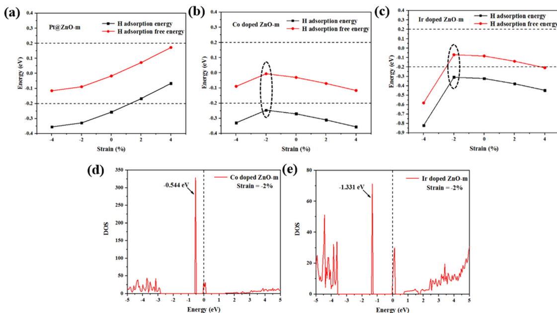
Fig. 6 Variation of the H adsorption energies and free energies as a function of (a) Pt@ZnO-m, (b) Co-doped ZnO-m, and (c) Ir-doped ZnO-m with strain. The DOS of (d) Co-doped ZnO-m with -2\% strain and (e) Ir-doped ZnO-m with -2\% strain. Vertical dashed lines represent the Fermi levels.
