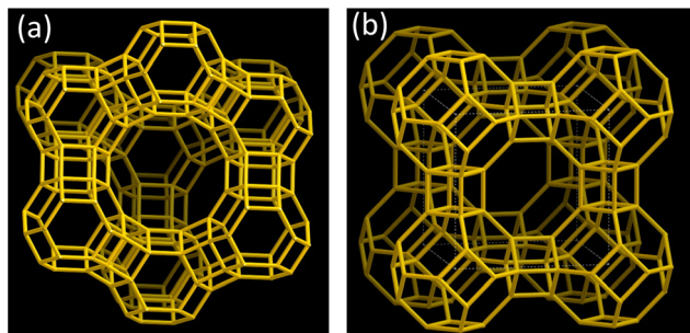
Fig. 3 Framework structure of (a) FAU and (b) LTA. 19 The Si–O–Si(Al) bonds are depicted as orange sticks.
