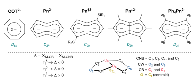
Fig. 1 Dianionic 10\pi ligands for organometallic complexes (upper) and positional numbering and hapticity definition of pentalenides (lower).
