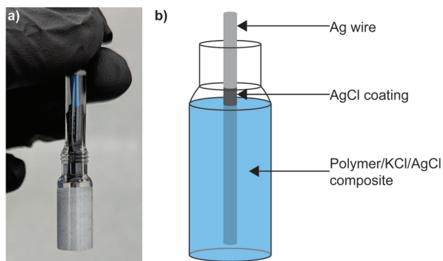
Fig. 1 (a) picture of KCl/AgCl SSRE, and (b) schematic illustrating the electrode's construction.
