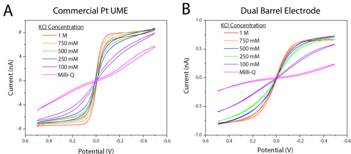
Fig. 6 Changes in voltammetry with changing salt concentration on a (A) commercial CHI platinum UME ( r = 5 \text{ } \mu\text{m} ) working electrode with a Pt wire quasi-reference counter electrode and (B) a dual barrel electrode (WE r = 0.59 \text{ } \mu\text{m} , QRCE r = 0.60 \text{ } \mu\text{m} ). Voltammetry was taken in a 5 mM potassium hexacyanoferrate(II/III) solution with changing salt concentration from 0.5 V to -0.5 V at a scan rate of 0.1 \text{ V s}^{-1} with a 2 seconds quiet time for 5 scans. The final scan for each voltammogram is plotted in polarographic convention.
