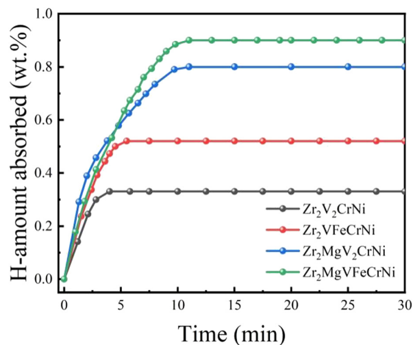
Fig. 5 Hydrogen absorption kinetics curves of \text{Zr}_2\text{Mg}_x\text{V}_{2-y}\text{Fe}_y\text{CrNi} ( x = 0 and 1, and y = 0 and 1) high-entropy alloys at 303 K.
