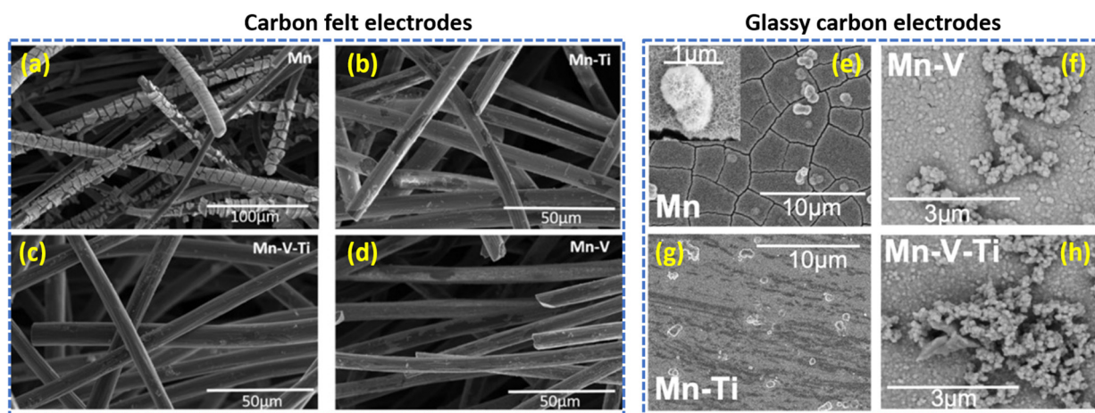
Fig. 11 SEM images of electrodeposited \text{MnO}_2 on the carbon felt electrodes (a)–(d) and on the glassy carbon electrodes (e)–(h), respectively (reproduced from ref. 74 with permission from Wiley-VCH).
