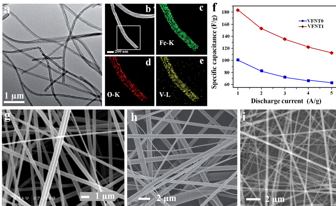
Fig. 13 (a) TEM microstructure \text{V}_2\text{O}_5/1 \text{ wt\% Fe}_2\text{O}_3 . (b)–(e) HAADF-STEM pattern and EDX mapping. (f) Variation of the specific capacitance of \text{V}_2\text{O}_5 (VFNT0) and \text{V}_2\text{O}_5/1 \text{ wt\% Fe}_2\text{O}_3 (VFNT1) at different current densities. Reproduced from ref. 109 with permission from Royal Society of Chemistry, copyright 2014. FE-SEM micrographs of electrospun fibers of: (g) \text{V}_2\text{O}_5 , reproduced from ref. 111 with permission from Royal Society of Chemistry, copyright 2010; (h) as-spun \text{V}_2\text{O}_5 nanofibers, reproduced from ref. 112 with permission from Wiley, copyright 2012 and (i) graphene oxide/ \text{V}_2\text{O}_5 nanofiber, reproduced from ref. 113 with permission from Elsevier, copyright 2014 respectively.
