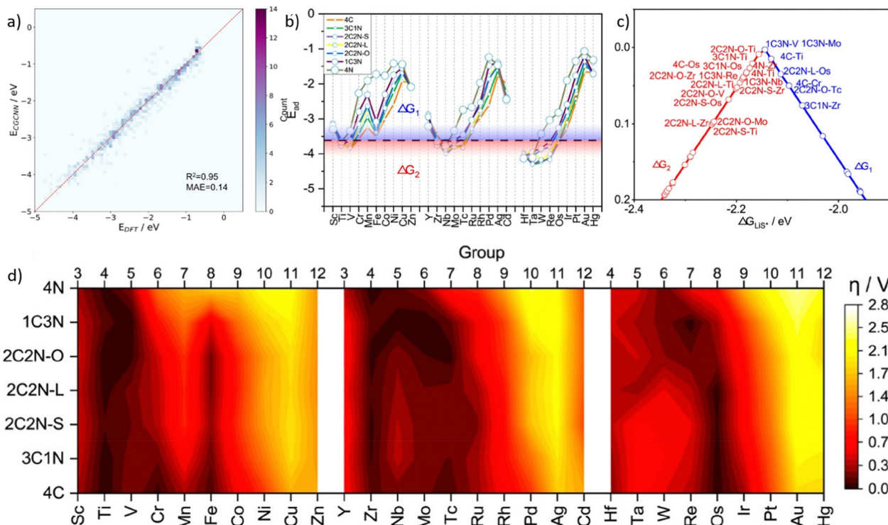
Fig. 10 Taken from Fig. 3 and 4 in Lian et al. 211 (a) DFT calculated and machine learning predicted adsorption energy of Li-polysulfides, (b) predicted adsorption energy of \text{LiS}^* , (c) volcano plots for catalysts with an overpotential lower than 0.1 V, and (d) heat map of the predicted overpotential of different SACs. Reproduced with permission. 211 Reprinted (adapted) with permission from ref. 211. Copyright 2021 American Chemical Society.
