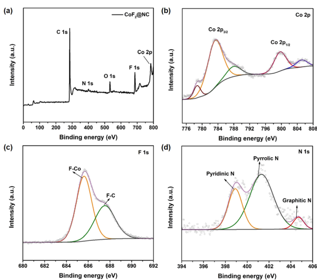
Fig. 2 (a) XPS survey spectrum of CoF 2 @NC. High-resolution XPS spectra of (b) Co 2p, (c) F 1s and (d) N 1s.
