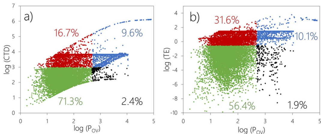
Fig. 1 Plots of CTD versus P_{OV} panel (a) and TE versus P_{OV} panel (b) from The Tool for 12 615 organic chemicals. The percentages of chemicals falling into each of the four quadrants are included. Chemicals identified as POP-like are located in the upper right quadrant (blue markers).
