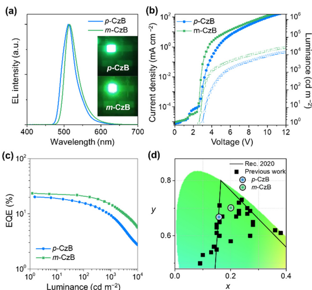
Fig. 4 EL characteristics of OLEDs that use p -CzB and m -CzB as MR-TADF emitters: (a) EL spectra and green EL images acquired at 10 mA \text{cm}^{-2} , (b) current density–voltage–luminance ( J - V - L ) characteristics, (c) EQE– L plots. (d) Comparing CIE coordinates for current and previously reported green OLEDs based on MR-TADF emitters (see ESI† for plotted data sets and source references).
