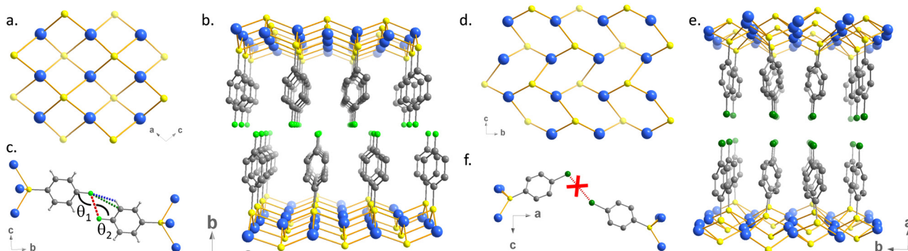
Fig. 2 Crystallographic structures of 1 and 2 , (a) representation of the (\text{AgS})_n network of 1 in the (a–c) plane, (b) central projection of the lamellar structure of 1 , (c) representation of the halogen interactions in 1 , the red dotted line is for \text{F} \cdots \text{F} = 2.965(2) \text{ \AA} , the green dotted line for \text{F} \cdots \text{C} = 3.391(5) \text{ \AA} and the blue dotted line for \text{F} \cdots \text{H} = 2.647(5) \text{ \AA} , (d) representation of the (\text{AgS})_n network of 2 on the (b–c) plane, (e) central projection of the lamellar structure of 2 and (f) view of the absence of halogen interaction in 2 . Blue spheres are for, Ag(I); yellow, S; light green, F; dark green, Cl and grey, C. Most hydrogen atoms are omitted for clarity.
