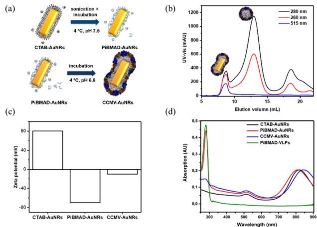
Fig. 3 (a) Schematic presentation the formation of CCMV-AuNRs mediated by PiBMAD; (b) FPLC analysis of CCMV-AuNRs; (c) Changes of zeta potential of AuNRs during the different coating steps; (d) UV-vis spectra of original CTAB-AuNRs, PiBMAD-AuNRs, CCMV-AuNRs, and PiBMAD-virus-like particles.
