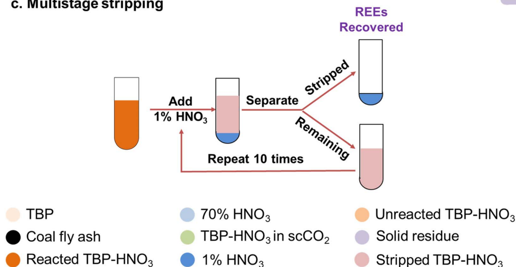
Fig. 1 Overview of processes for supercritical fluid extraction of REEs from solid CFAs. (a) Prepare extractant \text{TBP}-\text{HNO}_3 . (b) Extract REEs from CFAs using \text{TBP}-\text{HNO}_3 under SCF conditions and obtain the REEs-containing reacted \text{TBP}-\text{HNO}_3 . (c) Collect REEs and separate them from major impurities through a multistage stripping process.
