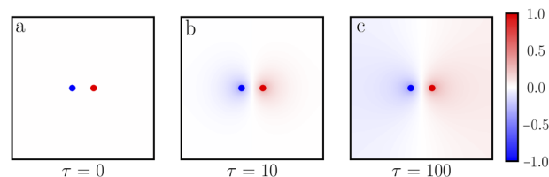
Fig. 8 Concentration field generated by a point source and sink dipole. (a–c) \tilde{c}(\mathbf{r}, \tau) at \tau = 0, 10, 100 for a dipole with d = 3 and a molar rate \mathcal{J}(\tau) = \mathcal{H}(\tau) . The color bar ranges between -1 and 1 and represents the value of \tilde{c}(\mathbf{r}, \tau) . The point source and sink are visualized as a red and blue circle and are not representative of solute concentration at the location of the source and sink.
