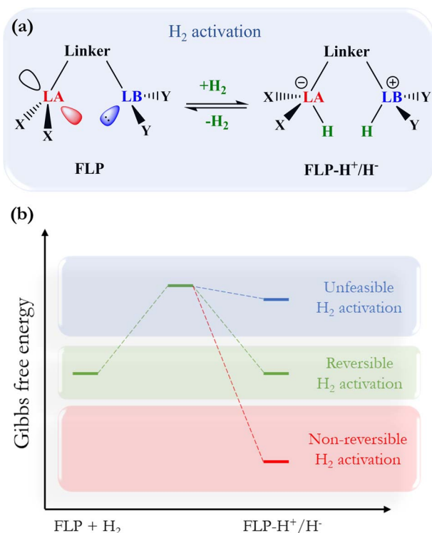
Fig. 1 (a) General scheme of \text{H}_2 activation by FLPs. (b) Energetic diagram for non-reversible, reversible, and a thermodynamically unfeasible \text{H}_2 activation by FLPs.
