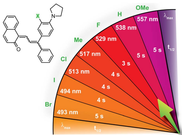
Fig. 7 Merocyanine color can be finely tuned by modulating the steric demand of the group adjacent to a para -pyrrolidine substituent. The \lambda_{\text{max}} and half-life ( t_{1/2} ) are given for merocyanines with various meta -substituents (X). Values shown were measured in toluene at 20 °C. 214
