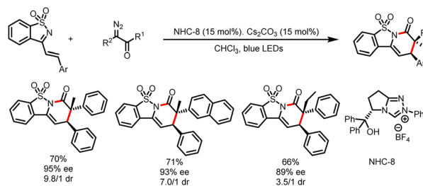
Scheme 22 Synthesis of dihydropyridinones.
