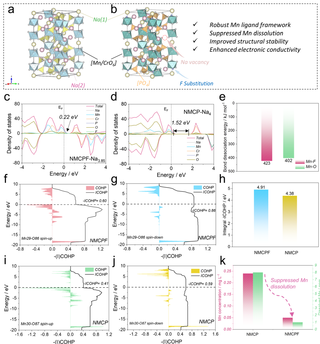
Fig. 1 Theoretical studies on the intrinsic physicochemical properties. Structural illustrations of (a) \text{Na}_4\text{MnCr}(\text{PO}_4)_3 and (b) F doped \text{Na}_4\text{MnCr}(\text{PO}_4)_3 . Total and partial DOS patterns of (c) NMCPF and (d) NMCP. (e) Bond dissociation energies of Mn–F and Mn–O. (f and g) COHP and ICOHP results of Mn29–O86 bond (spin-up and spin-down) in NMCPF. (h) Integral -ICOHP values of all Mn–O/F bonds in NMCPF and NMCP. (i and j) COHP and ICOHP results of Mn30–O87 bond (spin-up and spin-down) in NMCP. (k) Dissolved Mn concentrations in the electrolytes (claret-red) and separators (green).
