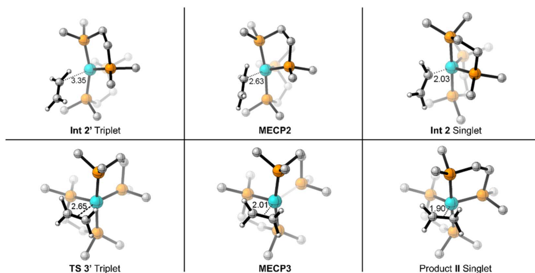
Fig. 3 3D depiction of M06-L optimized geometries for reaction between (\text{DMPE})_2\text{Fe} and ethylene with key bond/coordination distances (in Å).
